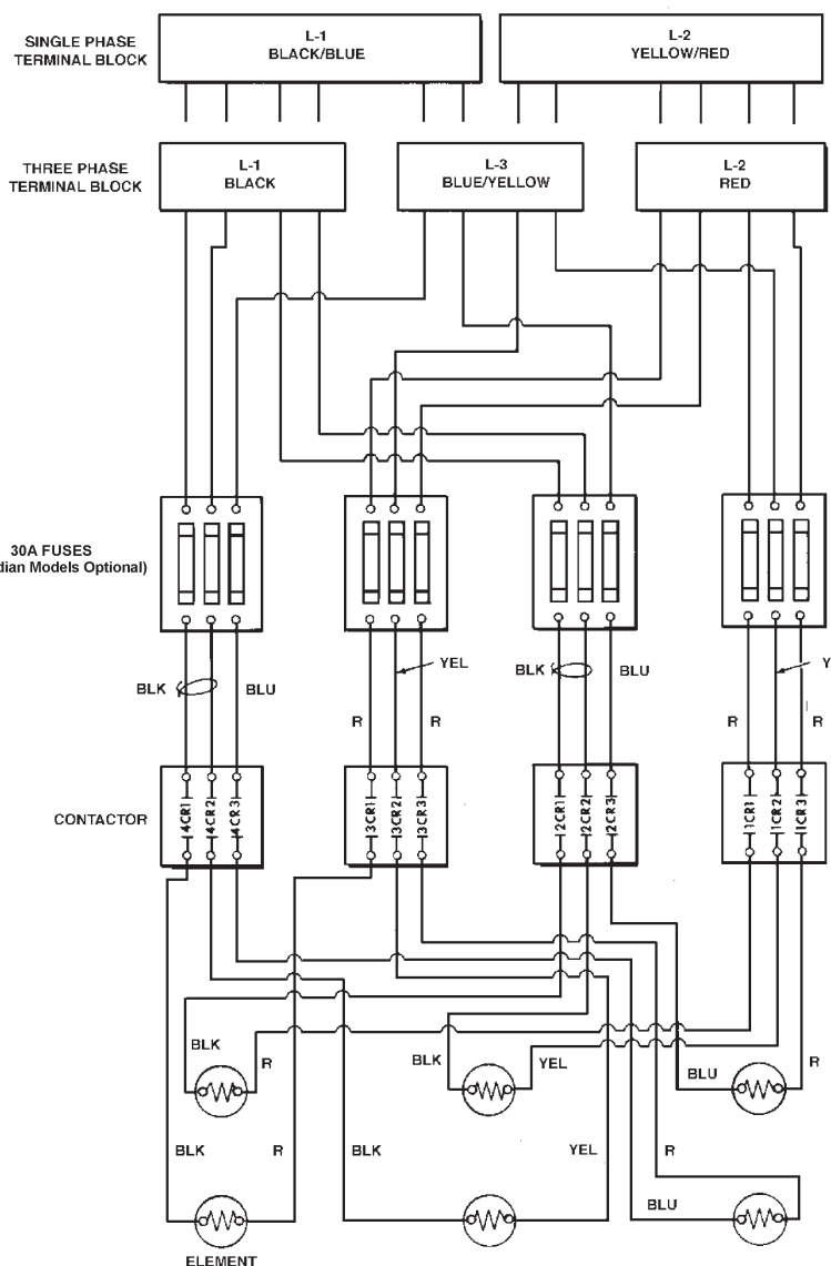
SIX ELEMENTS - SINGLE AND THREE PHASE
